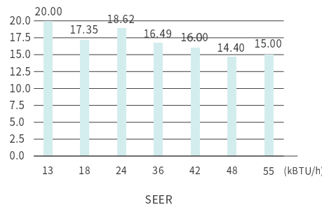
Cassette unit
